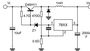
Fig.13 switching regulator
