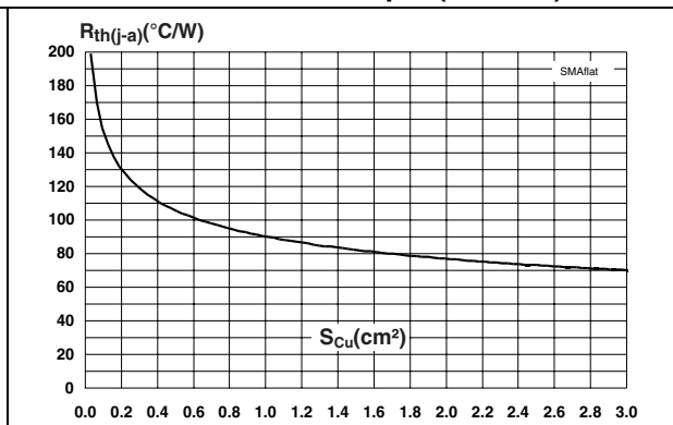
Figure 16. Thermal resistance junction to ambient versus copper surface under each lead - epoxy printed circuit board FR4, copper thickness = 35 \mu m (SMAflat)
