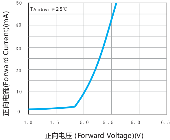
Volt-Ampere Characteristics
