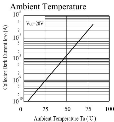
Fig.5 Collector Dark Current vs. Ambient Temperature
