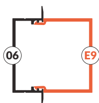
variant 06 - recessed 06-E9 wariant 06 - wpustowy 06-E9
