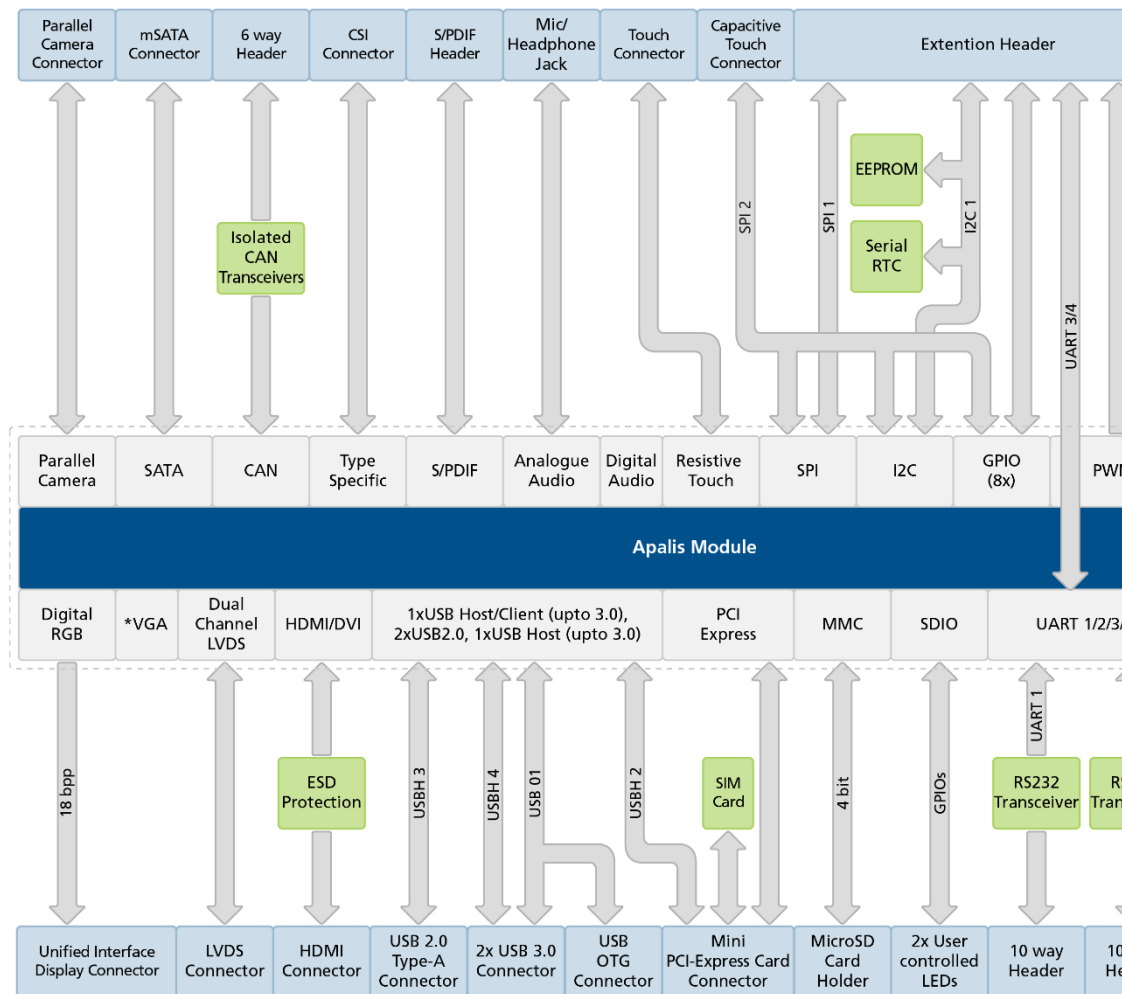
Fig.1 Ixora Carrier Board Hardware Architecture
