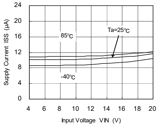
XC6202P332 (3.3V)
