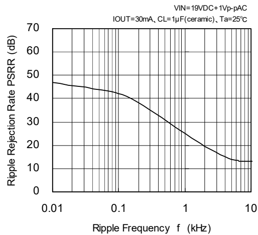
XC6202PJ02(18V)
