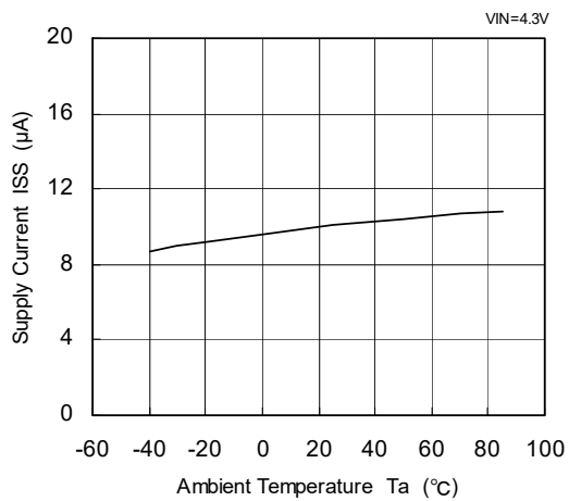
XC6202P332 (3.3V)
