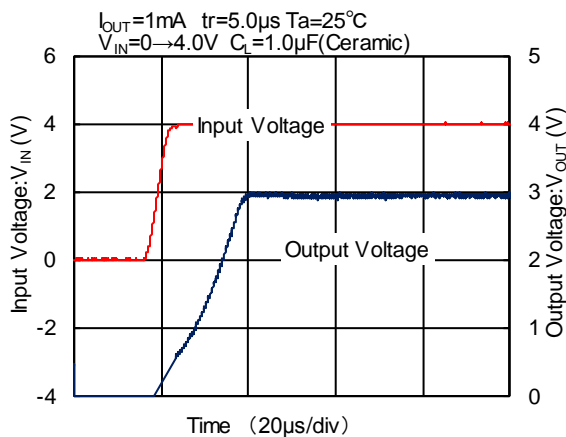
XC6231A302PR-G
