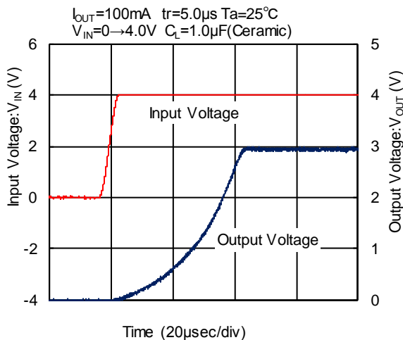
XC6231A302PR-G
