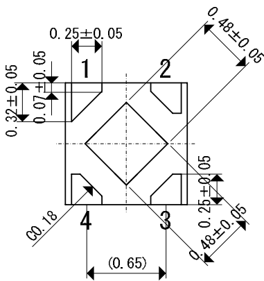
USPQ-4B04 Reference Pattern Layout (unit: mm)
