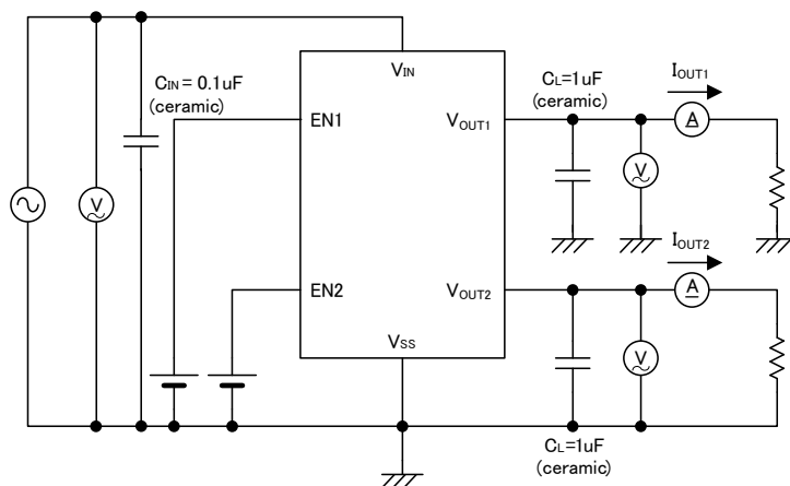
● Circuit ③
