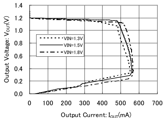
XC6601B121MR
