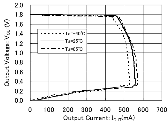
XC6601B181MR
