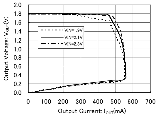
XC6601B181MR
