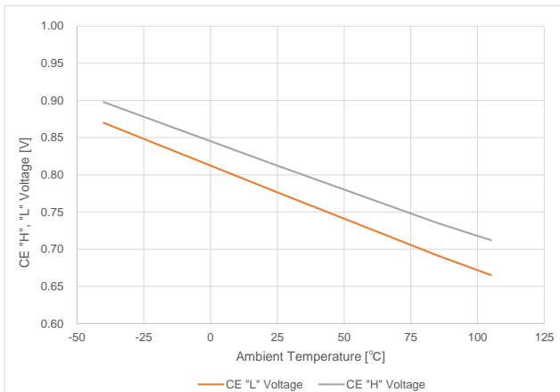
(11-3) CE "H", "L" Voltage vs Ambient Temperature XC8110/XC8111 Series
