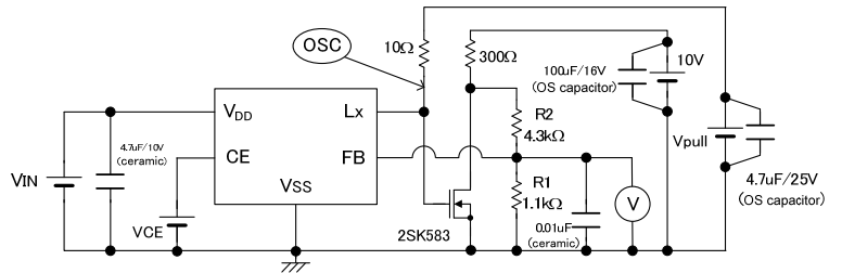
Circuit ④
