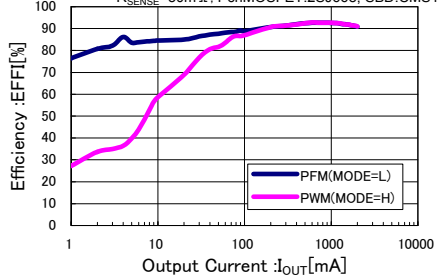
XC9252x08A( V_{IN}=24V , V_{OUT}=5.7V , f_{OSC}=280kHz )
