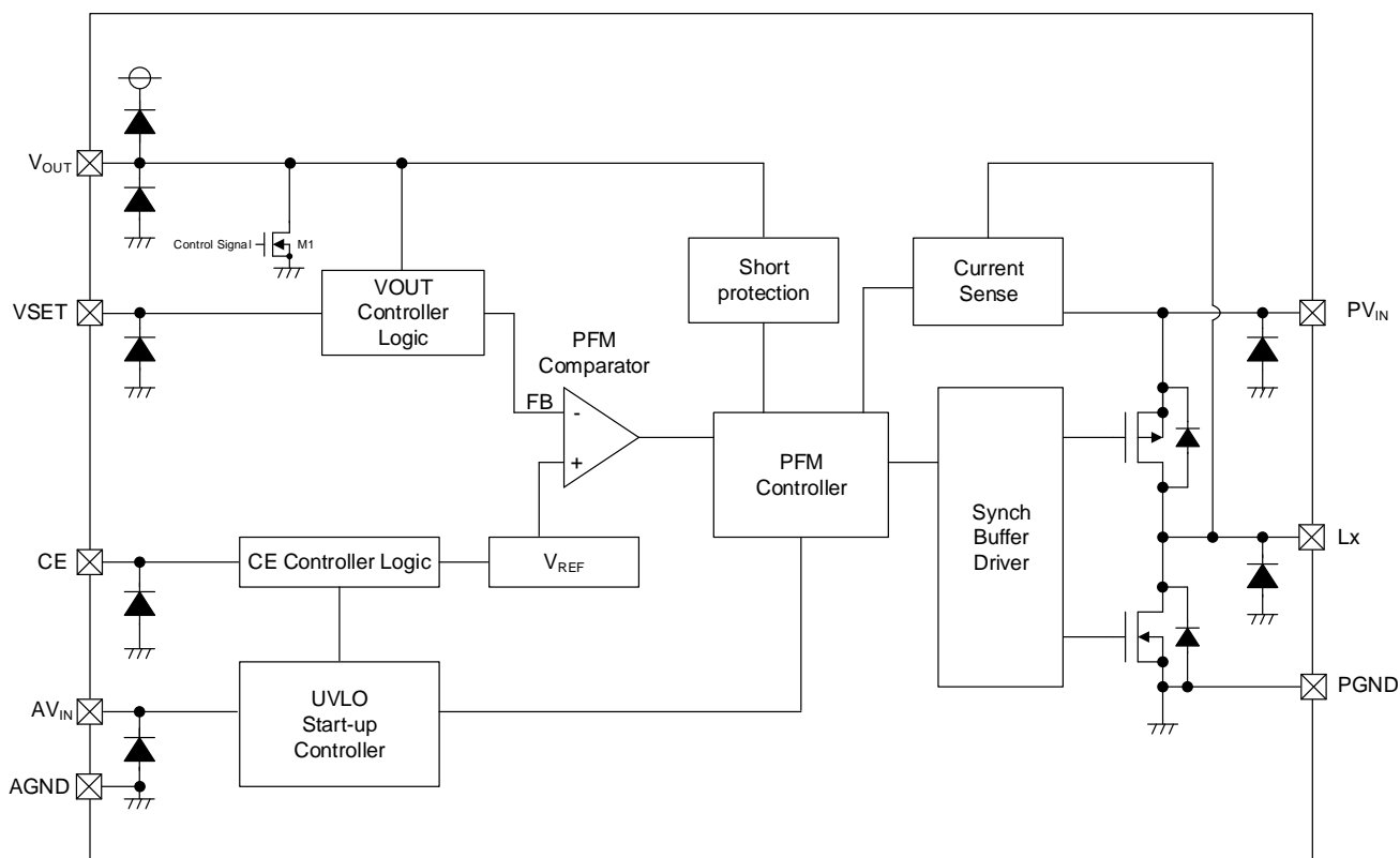
BLOCK DIAGRAM
