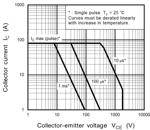
Fig. 8.9 Safe Operating Area (Guaranteed Maximum)
