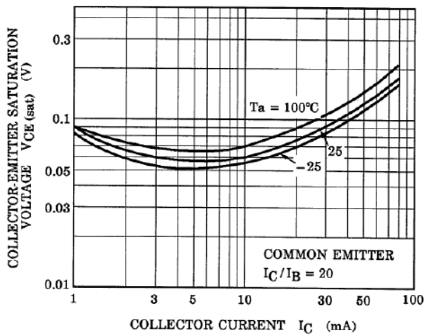
Fig. 10.21 RN1303 V_{CE(sat)}-I_C
