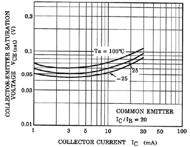
Fig. 10.22 RN1304 V_{CE(sat)}-I_C
