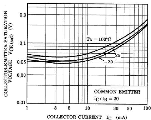
Fig. 10.23 RN1305 V_{CE(sat)}-I_C
