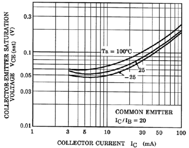
Fig. 10.20 RN1302 V_{CE(sat)}-I_C
