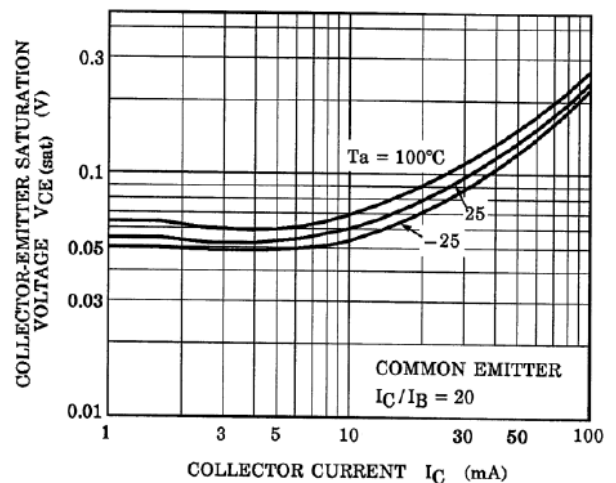
Fig. 10.24 RN1306 V_{CE(sat)}-I_C
