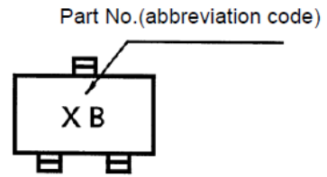
Fig. 9.2 Marking RN1302
