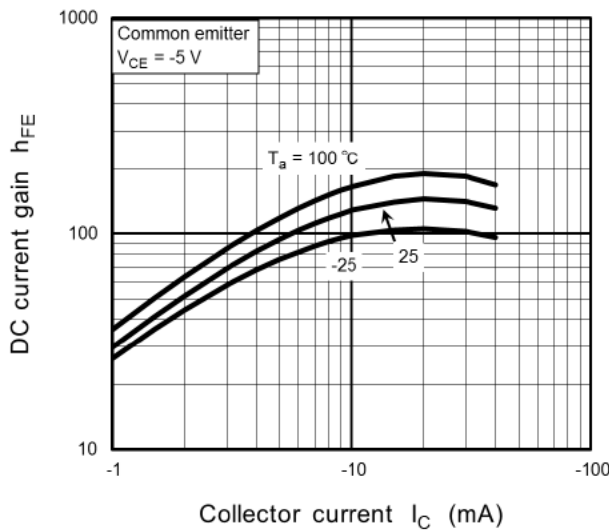
Fig. 11.15 RN2103MFV h_{FE} - I_C
