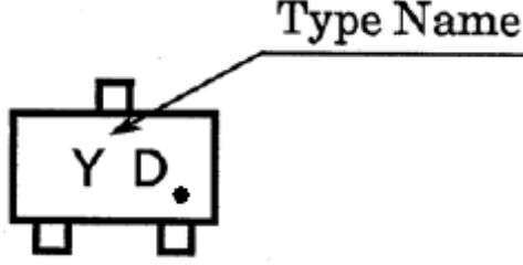
Fig. 10.4 Marking RN2104MFV
