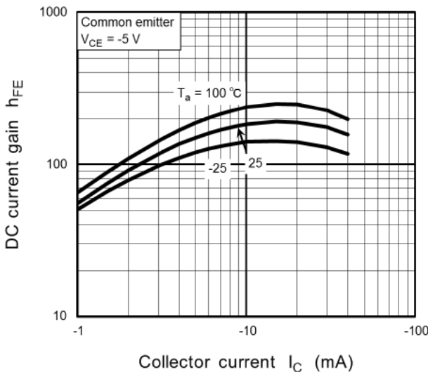
Fig. 11.17 RN2105MFV h_{FE(sat)} - I_C
