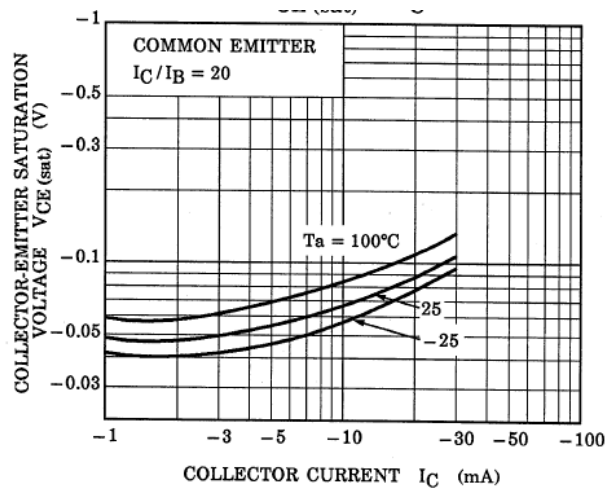
Fig. 10.22 RN2904 V_{CE(sat)}-I_C
