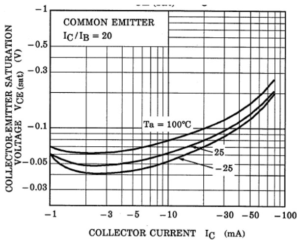
Fig. 10.21 RN2903 V_{CE(sat)}-I_C
