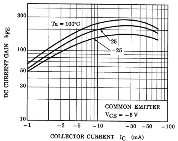
Fig. 10.16 RN2904 h_{FE-IC}
