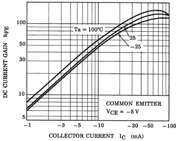
Fig. 10.13 RN2901 h_{FE-IC}
