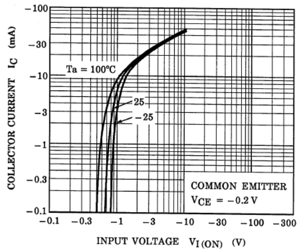
Fig. 10.6 RN2906 I_C - V_{I(ON)}
