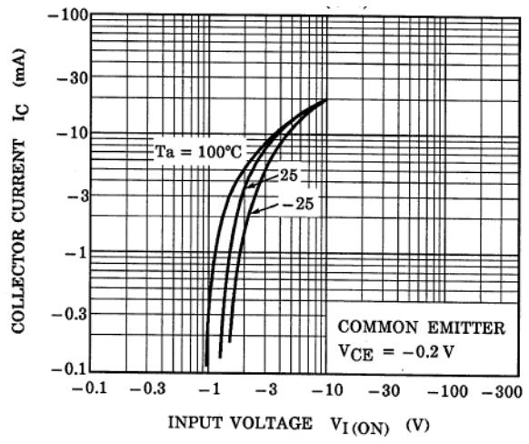
Fig. 10.4 RN2904 I_C - V_{I(ON)}
