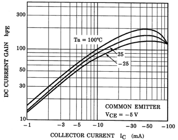
Fig. 10.14 RN2902 h_{FE-IC}
