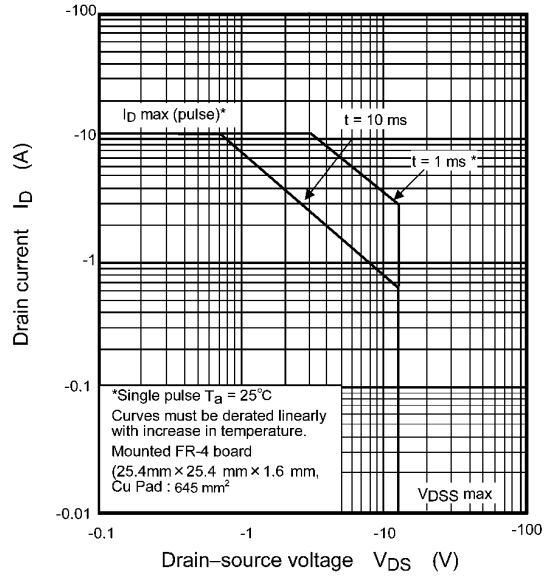
Fig. 7.14 Safe Operating Area
