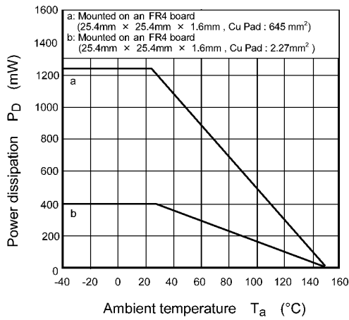
Fig. 8.15 P_D - T_a
