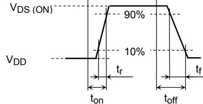
(c) V_{OUT}
