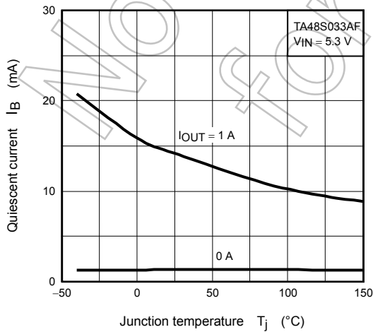
I_B - T_j
