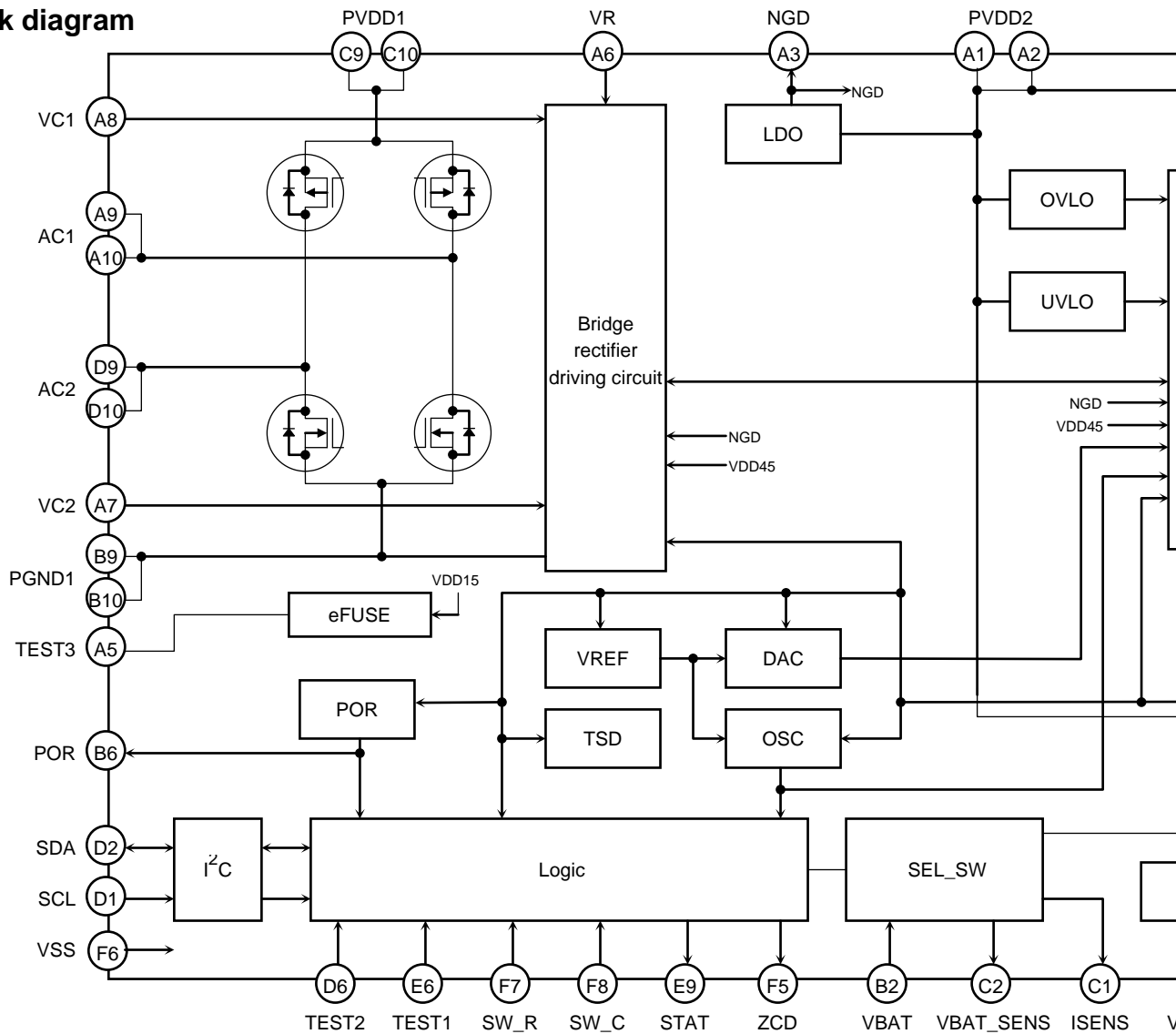
Figure 4.1 Block diagram
