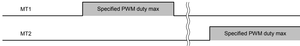
Figure 7.21 PWM Drive
