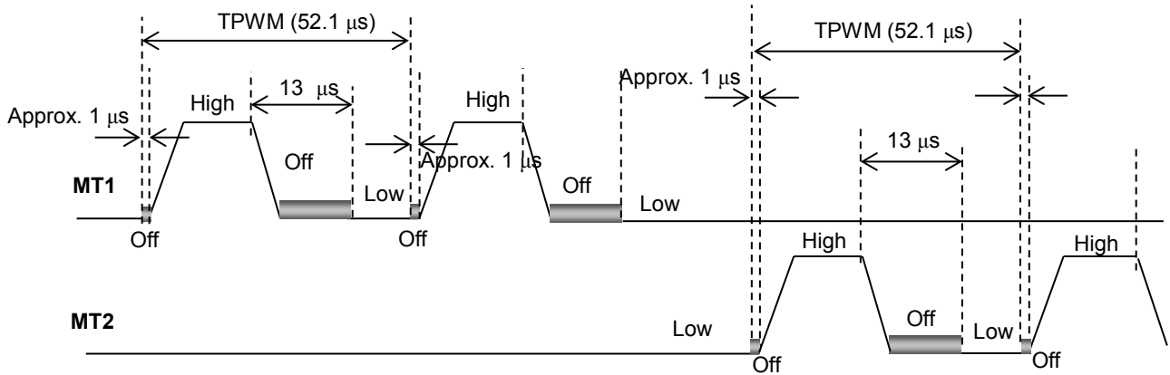
Figure 7.26 PWM Waveforms
