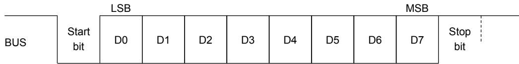
Figure 7.4 DATA Frame
