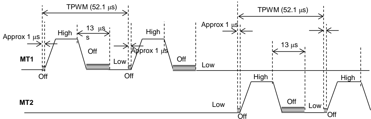
Figure 7.26 PWM Waveforms
