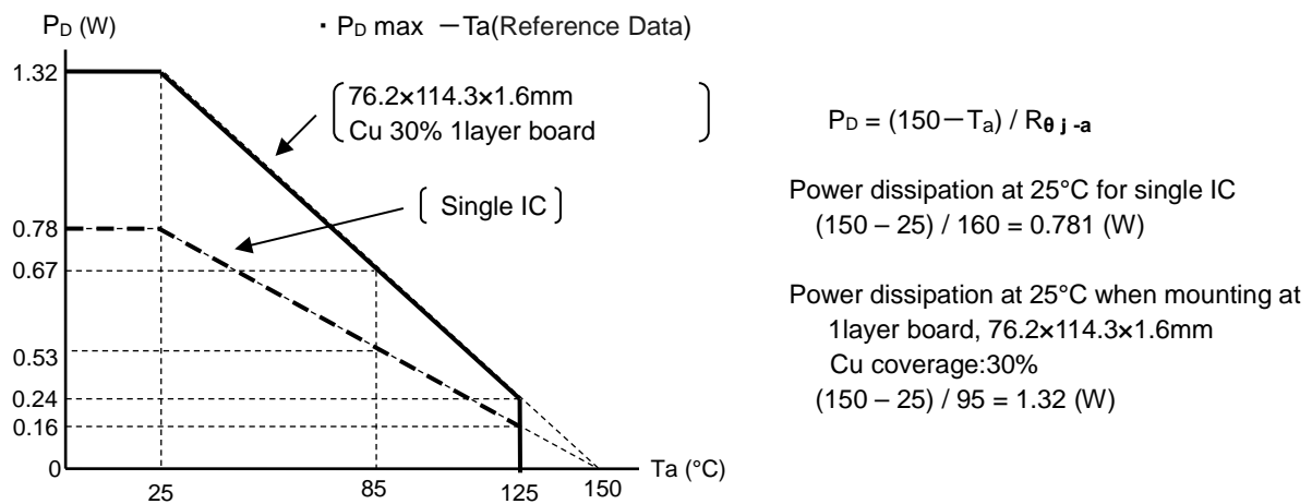
Figure 8.1 Thermal Characteristics
