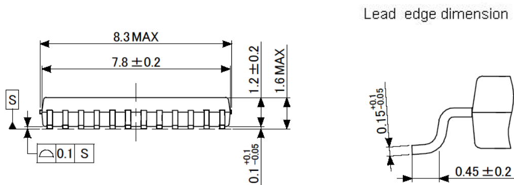
Figure 12.1 Package Dimensions
