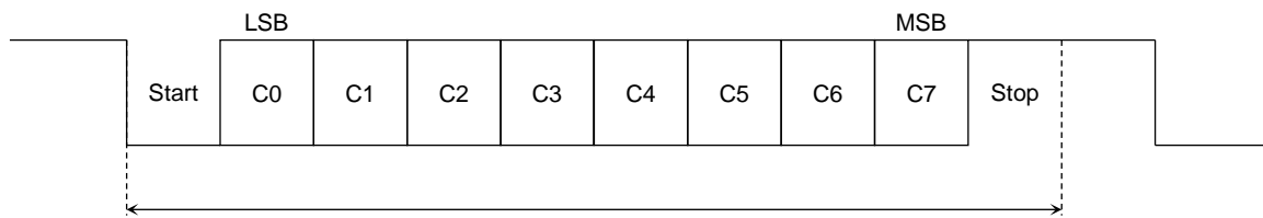
Figure 7.17 Checksum Field
