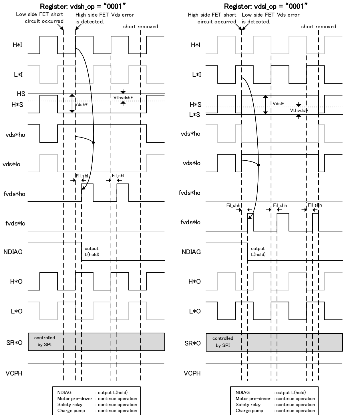
Fig. 7.5.8-c Timing chart for short-circuit detection (register vds_op = vds_op "0001")
