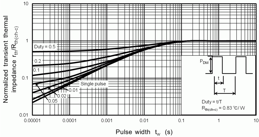
Fig. 8.18 r_{tr}/R_{th(ch-c)} - t_w (Guaranteed Maximum)
