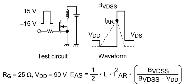
Fig. 8.16 Test Circuit/Waveform
