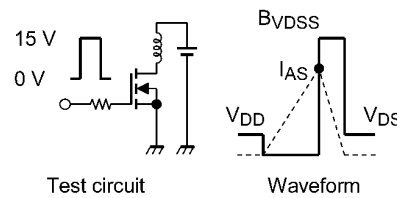
Fig. 8.16 Test Circuit/Waveform
