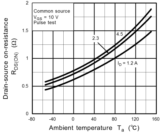
Fig. 8.7 R_{DS(ON)} - T_a
