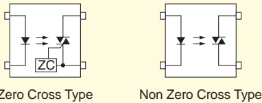
Zero Cross Type Non Zero Cross Type
