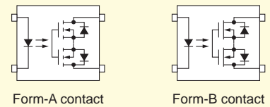
Form-A contact Form-B contact
