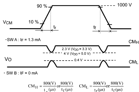
Fig. 12.1.6 Common-Mode Transient Immunity Test Circuit and Waveform
