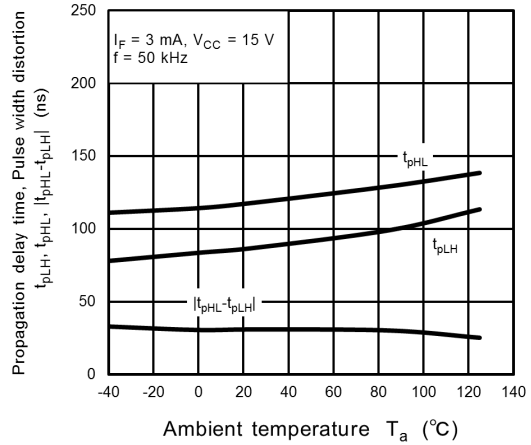
Fig. 12.2.22 t_{pHL}, t_{pLH}, |t_{pHL} - t_{pLH}| - T_a (Test Circuit Fig. 12.1.8)
