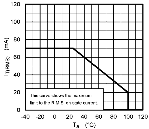
Fig. 12.2 I_{T(RMS)} - T_a
