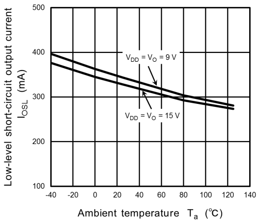
Fig. 12.2.9 I_{OL} - T_a
