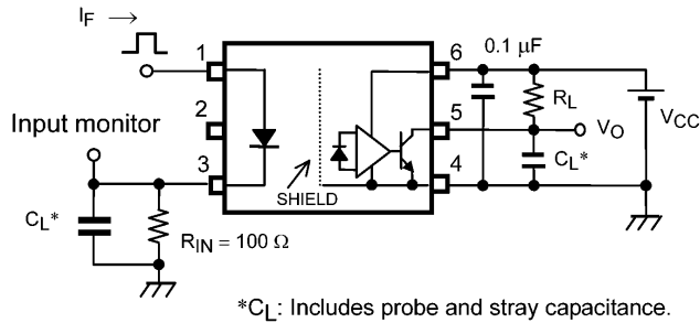
Fig. 13.1.5 Switching Time Test Circuit and Waveform
