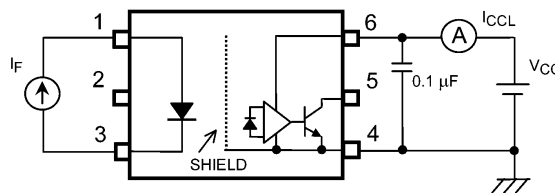
Fig. 13.1.4 I_{CCL} Test Circuit
