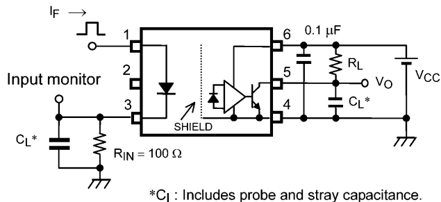
Fig. 13.1.5 Switching Time Test Circuit and Waveform
