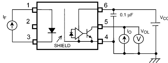
Fig. 13.1.2 V_{OL} Test Circuit
