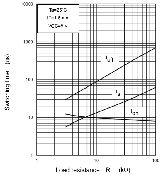
Switching time - R_L
