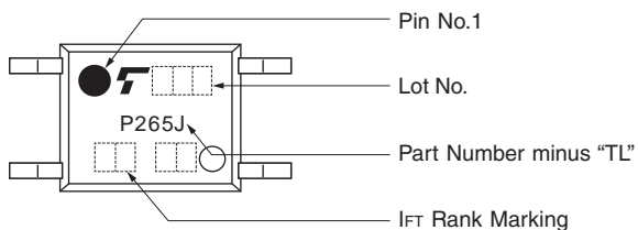
(a) 4 pin SO6 Package (TLP265J)
