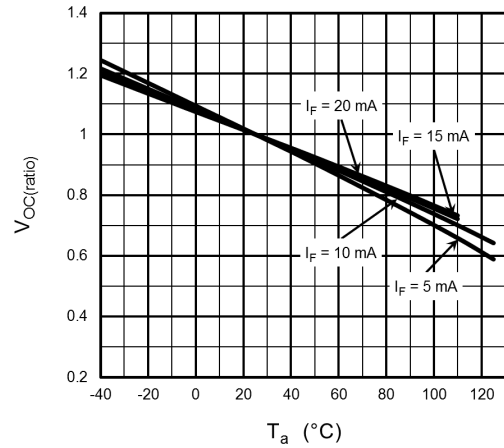
Fig. 12.8 V_{OC(ratio)} - T_a
