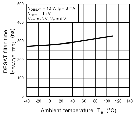
Fig. 13.3.36 t_{DESAT(FILTER)} - T_a
