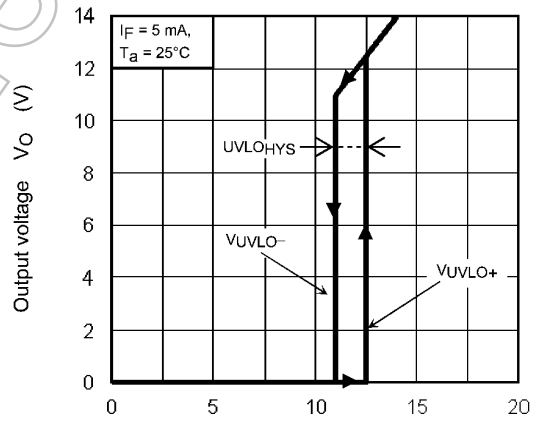
Fig. 12.2.12 V_O(V_{VLO}) - V_{CC}
