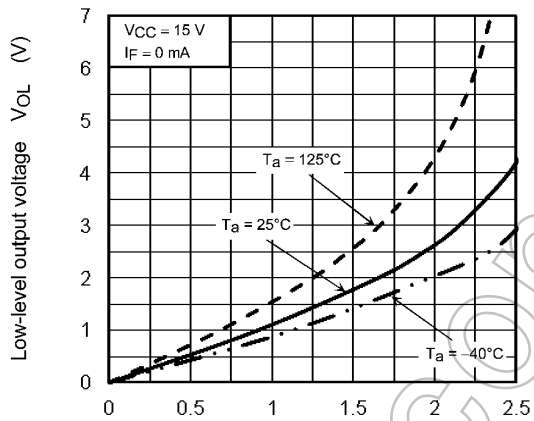
Fig. 12.2.9 V_{OL} - I_{OPL}
