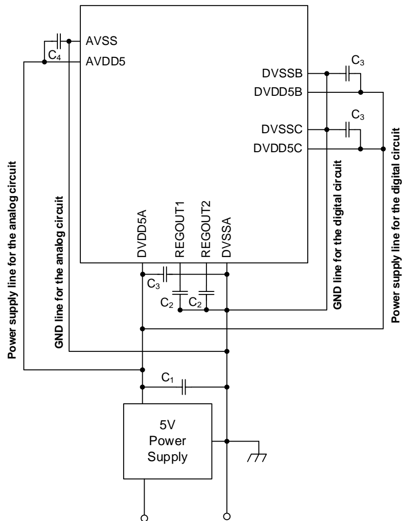
Figure 4.1 Capacitors between power supply pins
