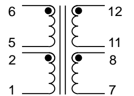
SCHEMATIC
