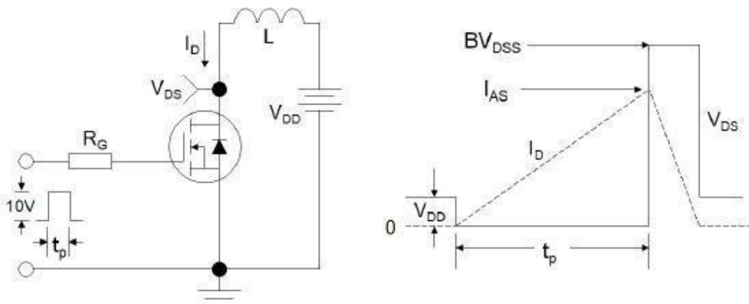
Figure 3:Unclamped Inductive Switching Test Circuit & Waveform
