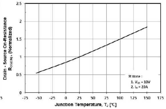
Fig. 8 On-Resistance Variation vs. Temperature
