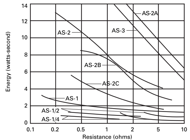
Selected Pulse-Handling Capability @ 125°C
