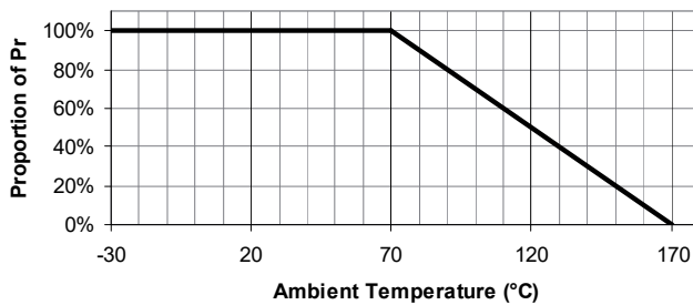
Temperature Derating
